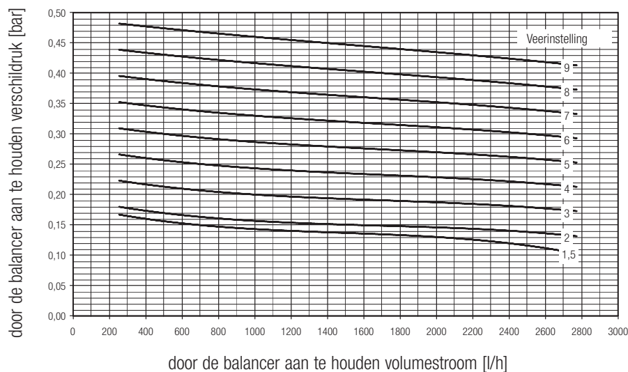
Instelcurven balancer G (DN 32)
