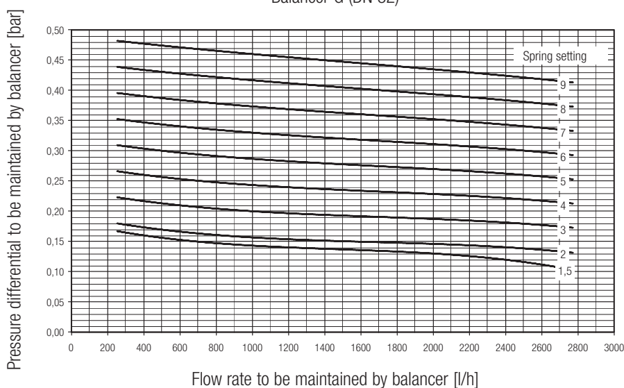
Setting curves Balancer G (DN 32)
